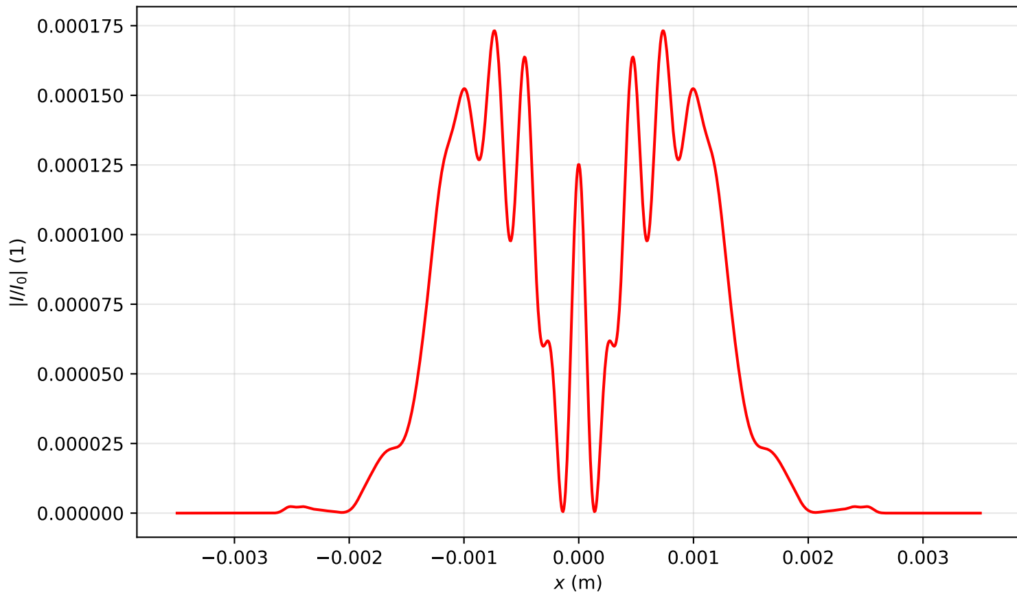
Intensity profile I(x, y = 0, z = 1.115)/I_0 , P_{in}=9.0P_{cr} , artificial time
